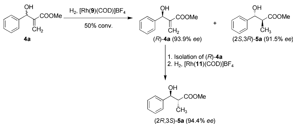
Scheme 4. Production of both enantiomers of 5a by two consecutive diastereoselective hydrogenations with different chiral catalysts.
