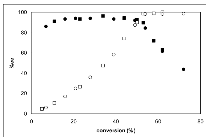
Figure 3. Selective hydrogenation of 4a (□/○) to anti - 5a (■/●) with [Rh( 9 )(COD)]BF 4 (●/○) and [Rh( 11 )(COD)]BF 4 (■/□) (15 bar, 25 °C, S/C = 200, THF).
