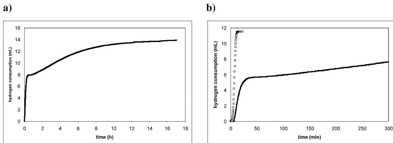
Figure 4. Consumption of hydrogen during the reaction of a) 4a with [\text{Rh}(\mathbf{9})(\text{COD})]\text{BF}_4 and b) 4c (bold line, continued up to 17 h with 11.5 mL \text{H}_2 consumption) and 4c ( \square ) with [\text{Rh}(\mathbf{9})(\text{COD})]\text{BF}_4 [S/C=100, 25 °C, \text{H}_2 (1 bar, isobar), 10 mL THF].
