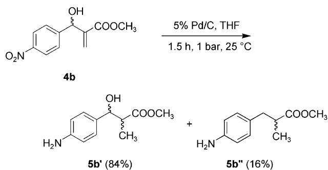
Scheme 3. Products of the heterogeneous Pd-catalyzed hydrogenation of 4b .
