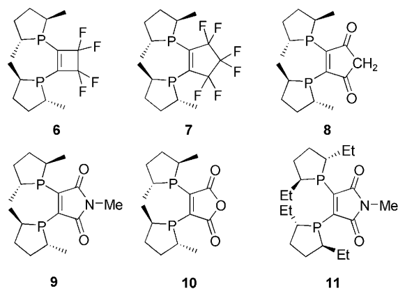
Figure 1. Structures of ligands 6–11 .
