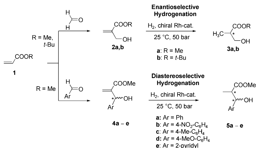
Scheme 1. Synthesis of functionalized olefins 2 and 4 by Baylis–Hillman reaction and their subsequent stereoselective hydrogenation.
