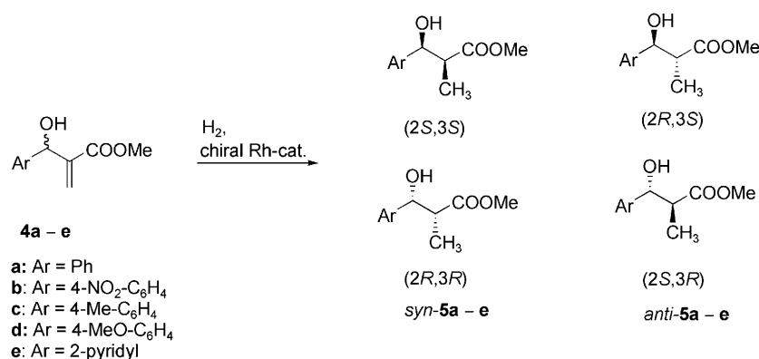
Scheme 2. Possible hydrogenation products derived from 4a–e .
