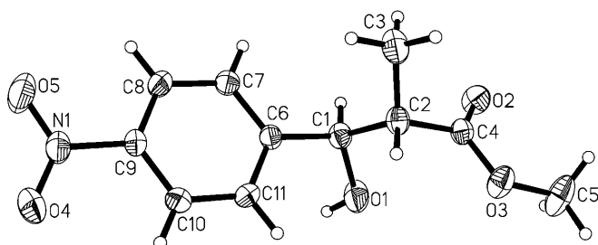
Figure 2. X-ray structural analysis of anti - 5b . The thermal ellipsoids correspond to 30% probability.
